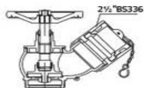
(THREAD TYPE)
